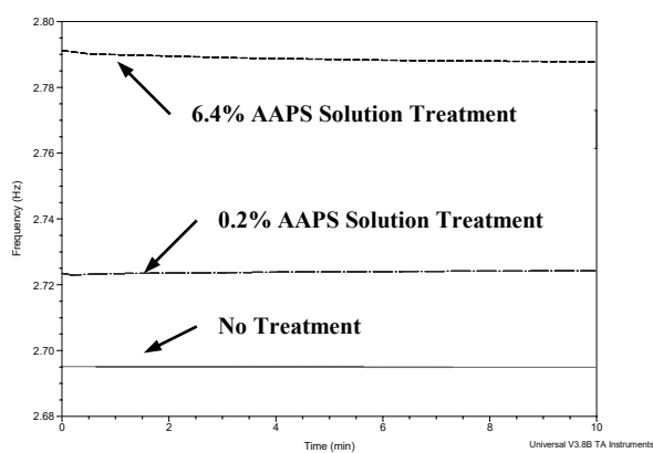
Figure 3. Resonant mode DMA (frequency vs. time) for a 6.4% AAPS treated steel-core string, a 0.2% AAPS treated steel-core string, and an untreated steel-core string.
